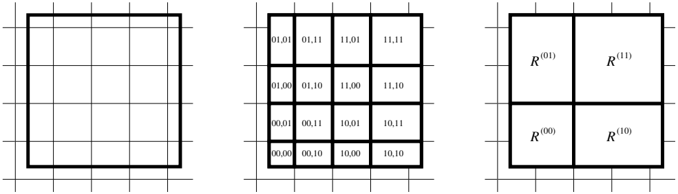
Figure 2. (i) Cube Q and Q_{i-1,u} -grid; (ii) basic rectangles; (iii) level-1 rectangles.
