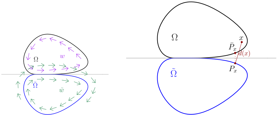
Figure 2. Vector fields w and \tilde{w} , and d(x), P_x, \bar{P}_x for x \in \Omega .
