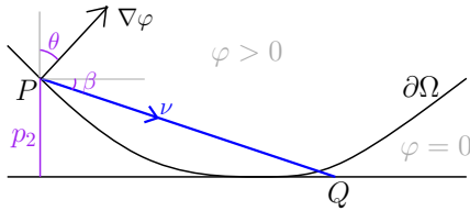
Figure 3. The definitions of \theta, \beta, \nu, Q .
