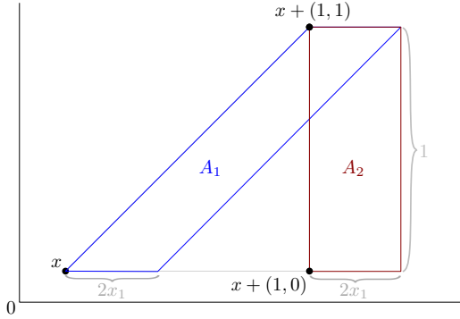
Figure 8. The domains A_1 and A_2 .
