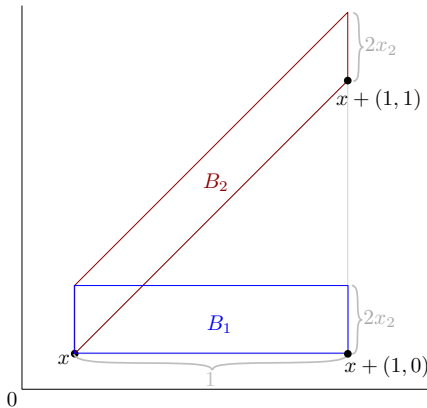
Figure 9. The domains B_1 and B_2 .
