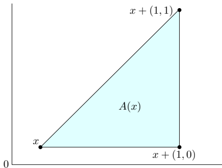
Figure 7. The domain A(x) .
