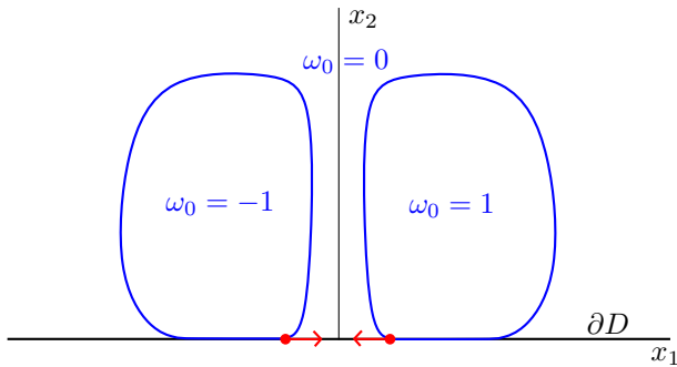
Figure 1. Initial data \omega_0 that leads to a finite time singularity.
