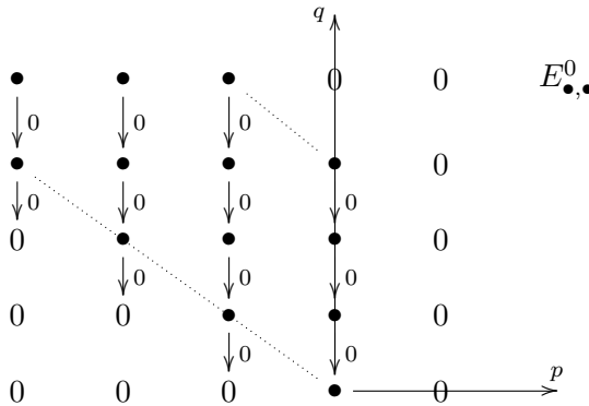
Figure 3.1. Zeroth term E_{\bullet,\bullet}^0 of the spectral sequence. The dotted lines indicate the limits wherein the spectral sequence is concentrated.
