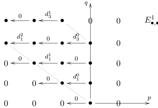
Figure 3.2. First term E_{\bullet, \bullet}^1 of the spectral sequence.
