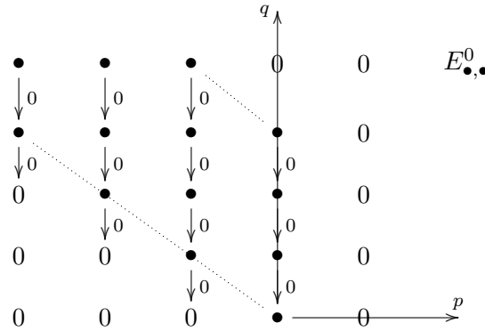
Figure 3.1. Zeroth term E_{\bullet,\bullet}^0 of the spectral sequence. The dotted lines indicate the limits wherein the spectral sequence is concentrated.
