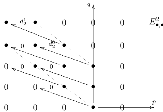
Figure 3.3. Step E_{\bullet, \bullet}^2 of the spectral sequence.
