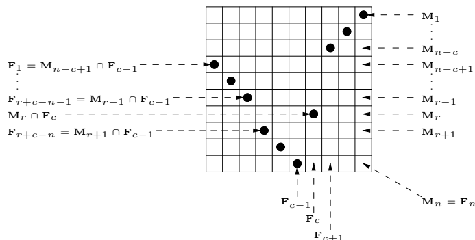
Figure 6: A convenient description of a double Schubert cell in the specialization order in terms of transverse \{\mathbf{F}_c, \dots, \mathbf{F}_n\} and \mathbf{M}_\bullet , and \mathbf{F}_{c-1} in given position with respect to \mathbf{M}_\bullet . Some squares of the checkerboard are labeled with their corresponding vector space.
