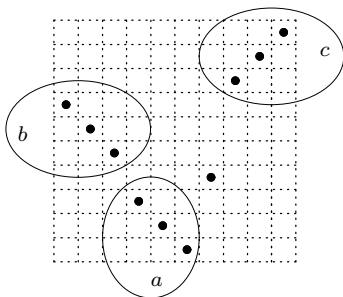
Figure 24: The corresponding point in the checkergame
