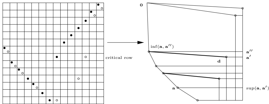
Figure 18: An example of \mathcal{Q}_\circ for mid-sort \circ . The internal diagonal edges of the region \inf(\mathbf{a}, \mathbf{a}'')\mathbf{a}'\sup(\mathbf{a}, \mathbf{a}')\mathbf{a} are thickened.
