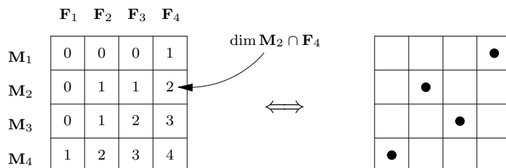
Figure 4: The relative positions of two flags, given by a rank table, and by a configuration of black checkers.
