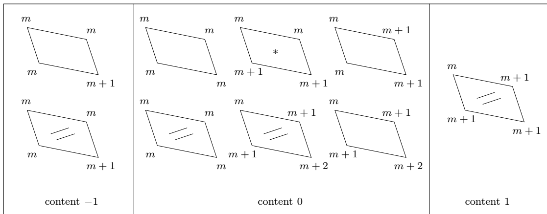
Figure 17: Possible labeled quadrilaterals, where \mathbf{c} is labeled with \dim V_{\mathbf{c}} \cap Z for some fixed vector space Z . Quadrilateral * arises in Lemma 5.5.
