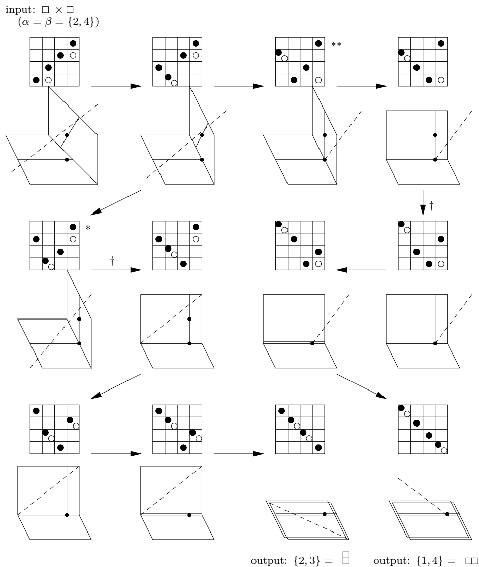
Figure 3: A motivating example of the rule (compare to Figure 2). Checker configurations * and ** are discussed in Caution 2.20, and the degenerations labeled † are discussed in Sections 2.11 and 3.1.
