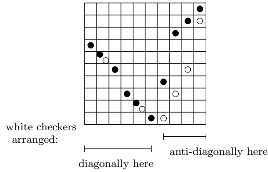
Figure 7: An example of mid-sort checkers
