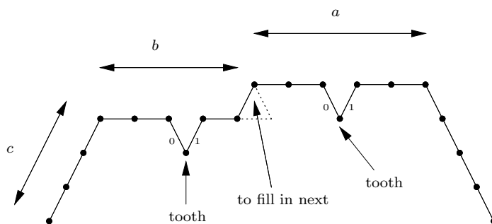
Figure 23: The puzzle in the process of being filled
