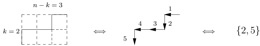
Figure 1: The bijection between \text{Rec}_{k,n-k} and size k subsets of \{1, \dots, n\} .
