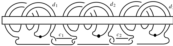
Figure 8.4. Before the last (g - 1) cancellations.
