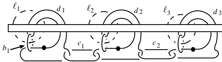
Figure 8.3. A 0-framed handle decomposition for \mathcal{S}^0K .
