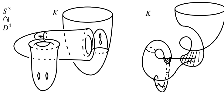
Figure 1.1. A grope of height 2.5 and a Whitney tower of height 2.5.
