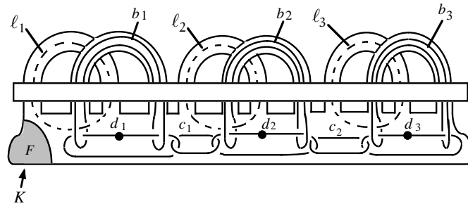
Figure 8.2. The cobordism C .
