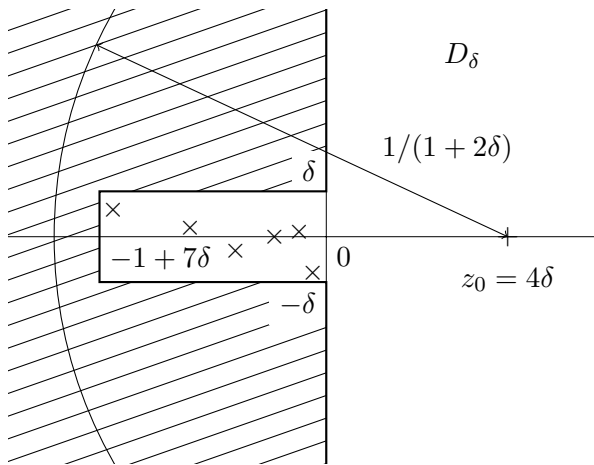
Figure 1. The domain D_\delta . Possible poles of F (marked with \times ) are located in D_\delta \cap \Re z \leq 0 .
