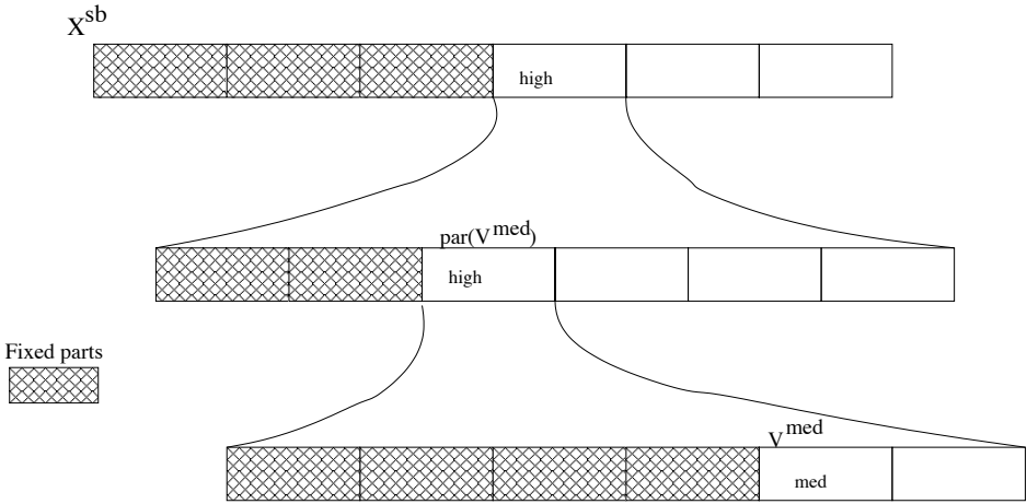
Figure 2. Finding a medium part in X^{\text{sb}} .
