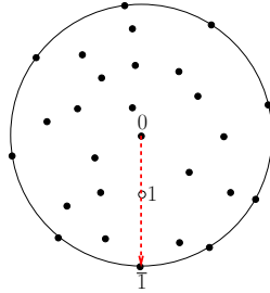
Figure 2. A general configuration of points in \overset{\circ}{\mathcal{Y}}_{n+1,m+1}^+ .
