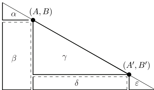
Figure 2.2. The subdivision of the triangle T_{A,B}^a .
