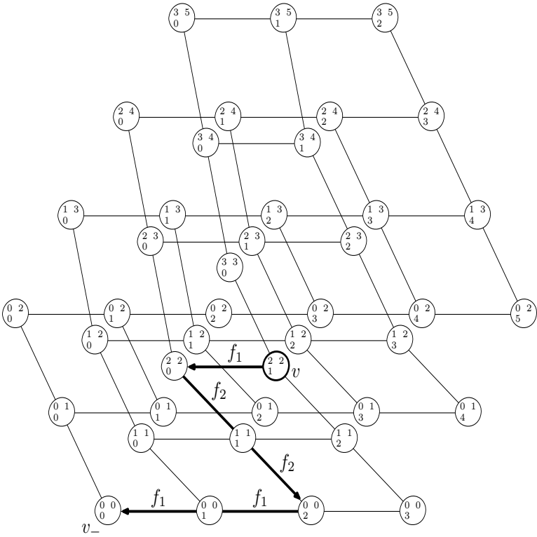
Figure 1. Starting with the vertex v , showing the canonical path to v_- , with respect to the word \Sigma_2 = (1, 2, 1) . The lengths of the three straight segments, 1, 2, 2 comprise the values in BZL(v) = \begin{pmatrix} 2 & 2 \\ 1 & 1 \end{pmatrix} . In this example, wt(v_-) = (0, 3, 5) and wt(v) = (3, 2, 3) .
