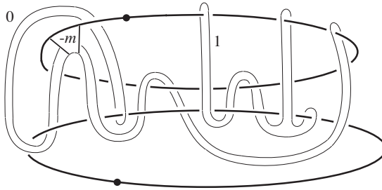
Figure 1. \Sigma_m
