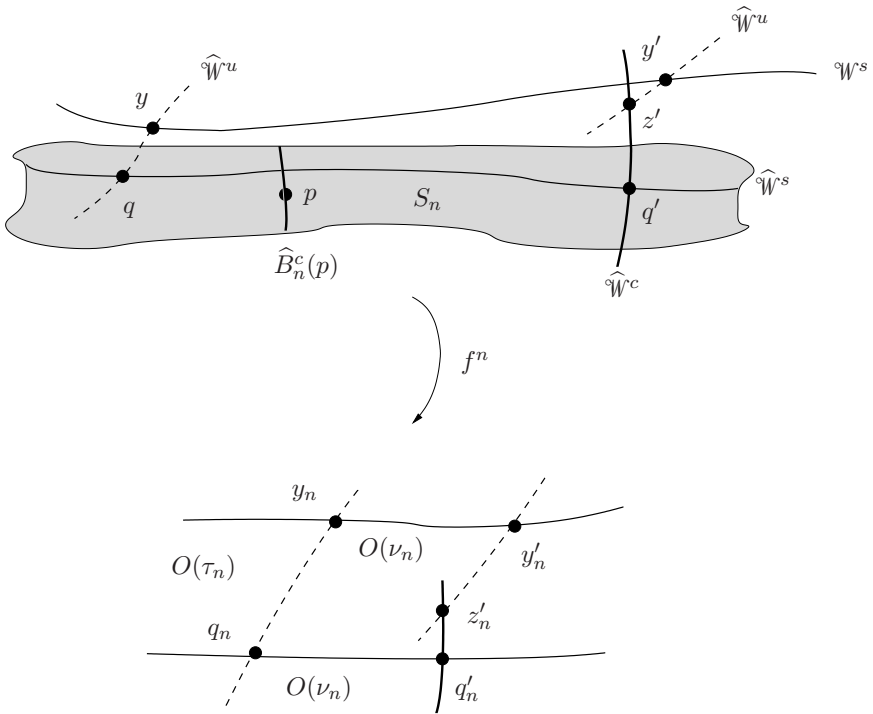
Figure 3. Picture for the proof of Lemma 6.2 .
