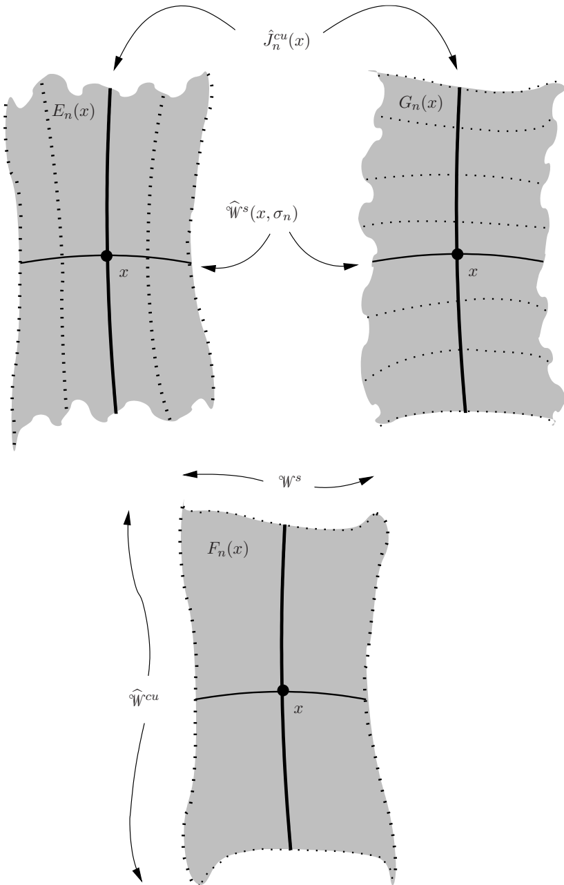
Figure 4. Comparison between E_n(x) , F_n(x) and G_n(x) .
