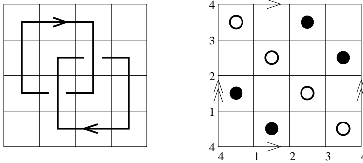
Figure 9: Grid presentation of the Hopf link.
