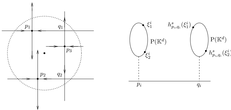
Figure 2: Stable holonomies
