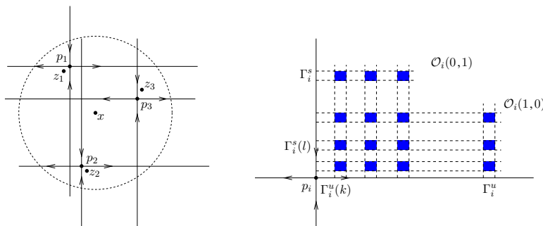
Figure 1: Extended holonomy block
